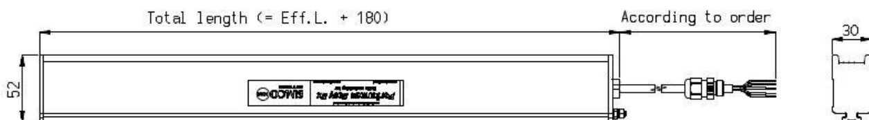
Image 4.1 : Dimensions du Performax IQ Easy Ex (Speed)
